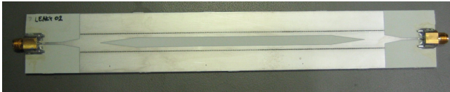
(b) 2-port SIW leaky wave antenna.
