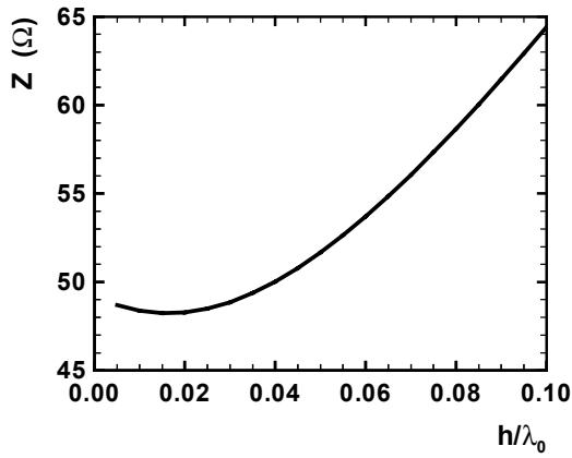
Fig. 4 The characteristic impedance of the microstrip line specified in Fig. 3.
