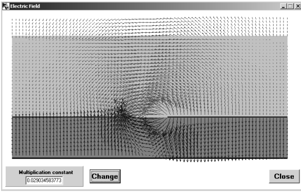
Fig. 16 Electric field of the dominant bound mode on the cross-sectional plane of the modified conductor-backed slotline specified in Fig. 12.
