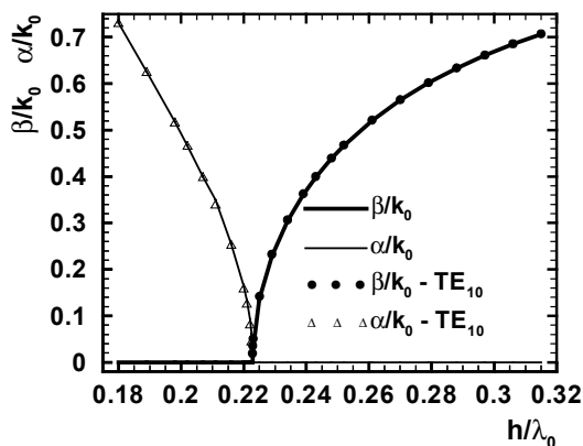
Fig. 21 The dispersion characteristic of the mode on the slotted rectangular waveguide compared with the characteristic of TE 10 mode. The slot width is 1 mm, and the internal dimensions are 22.86 x 10.12 mm.
