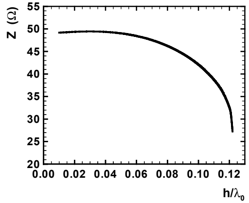
Fig. 13 Characteristic impedance of the coplanar waveguide specified in Fig. 12.
