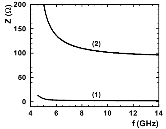
Fig. 18 The characteristic impedance (1) of the line specified in Fig.15 with the slot type mode, and (2) of the line when w=1 mm, 2h=10 mm, b=23 mm, \epsilon_r=1 , on which the slot type mode propagates.
