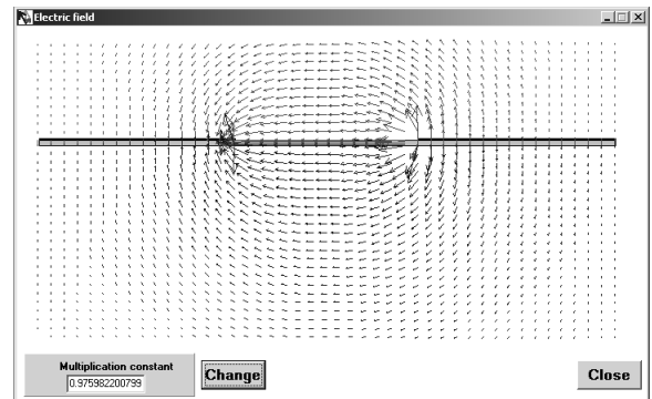
Fig. 9 Electric field of the even dominant bound mode on the slotline specified in Fig. 6 at h/\lambda_0=0.012 .
