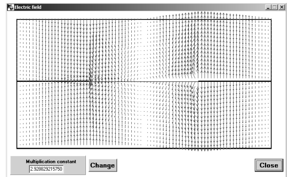
Fig. 19 Electric field of the even slot type dominant mode on a cross-sectional plane of the wide slotted line specified in Fig. 17 at f=7.5 GHz.
