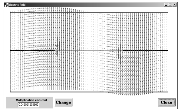
Fig. 20 Electric field of an even perturbed waveguide type mode on the cross-sectional plane of the wide slotted line specified in Fig. 17 at f=7.5 GHz.
