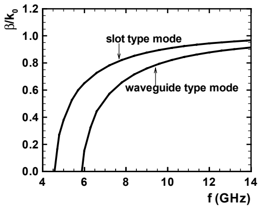
Fig.17 Normalized phase constant of the even dominant slot type mode, and waveguide type mode on a shielded conductor-backed slotline, ⑬ in Fig. 1, when slot width w=20 mm, height of the shield 2h=4 mm, its width b=50 mm and permittivity \epsilon_r=1 .
