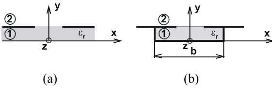
Fig. 2 Cross-section of a slotline (a) and a conductor-backed slotline with finite width of the substrate metallized on the side walls (b).
