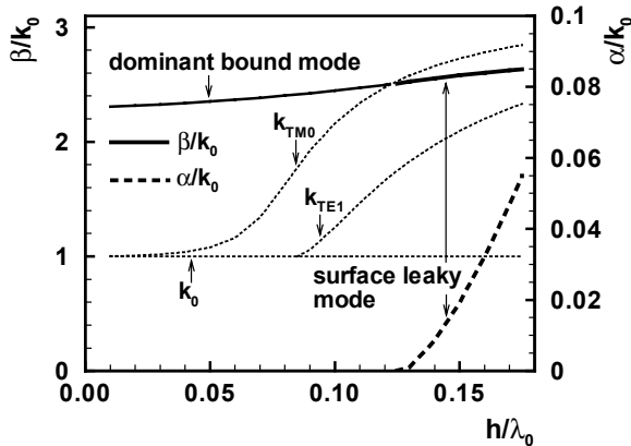
Fig. 12 Dispersion characteristics of a coplanar waveguide, ④ in Fig. 1, when central strip width s=0.6 mm, slot width w=0.25 mm, substrate thickness h=1 mm and permittivity \epsilon_r=10 .
