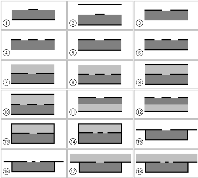
Fig. 1 Cross-sections of planar transmission lines analyzed by the APTL program.
