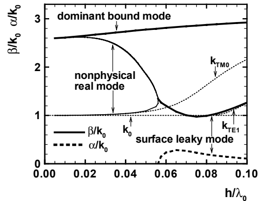
Fig. 3 Dispersion characteristics of the microstrip line, \textcircled{1} in Fig. 1, with strip width w=0.6 mm, substrate thickness h=0.635 mm and permittivity \epsilon_r=10 .
