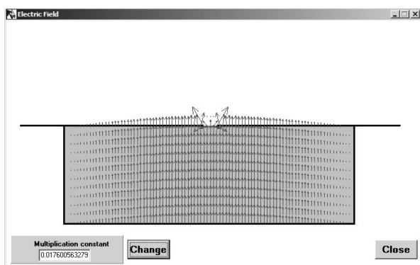
Fig. 22 Electric field of the mode on the slotted waveguide specified in Fig. 21.
