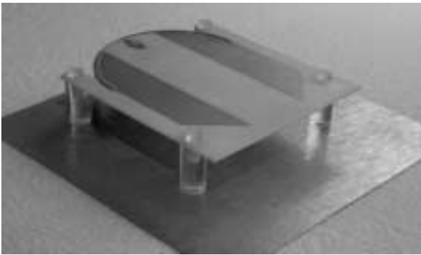
Fig. 7 The fabricated flat top leaky wave antenna.
